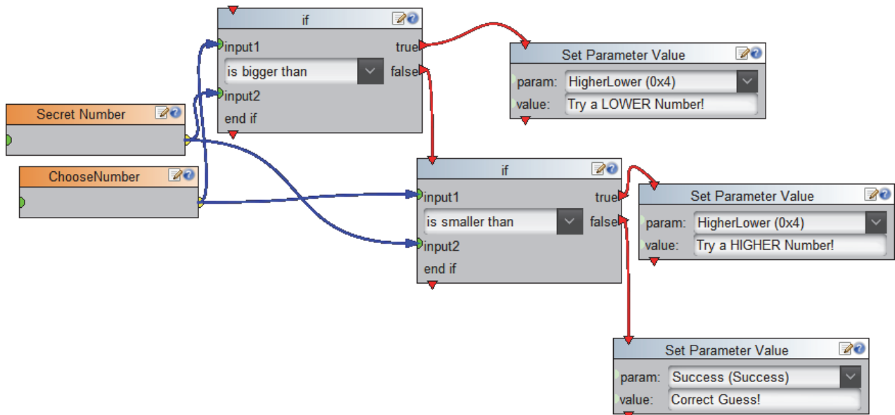
Figure 6.4 - The if Logic Block Connected to Other Logic Blocks
