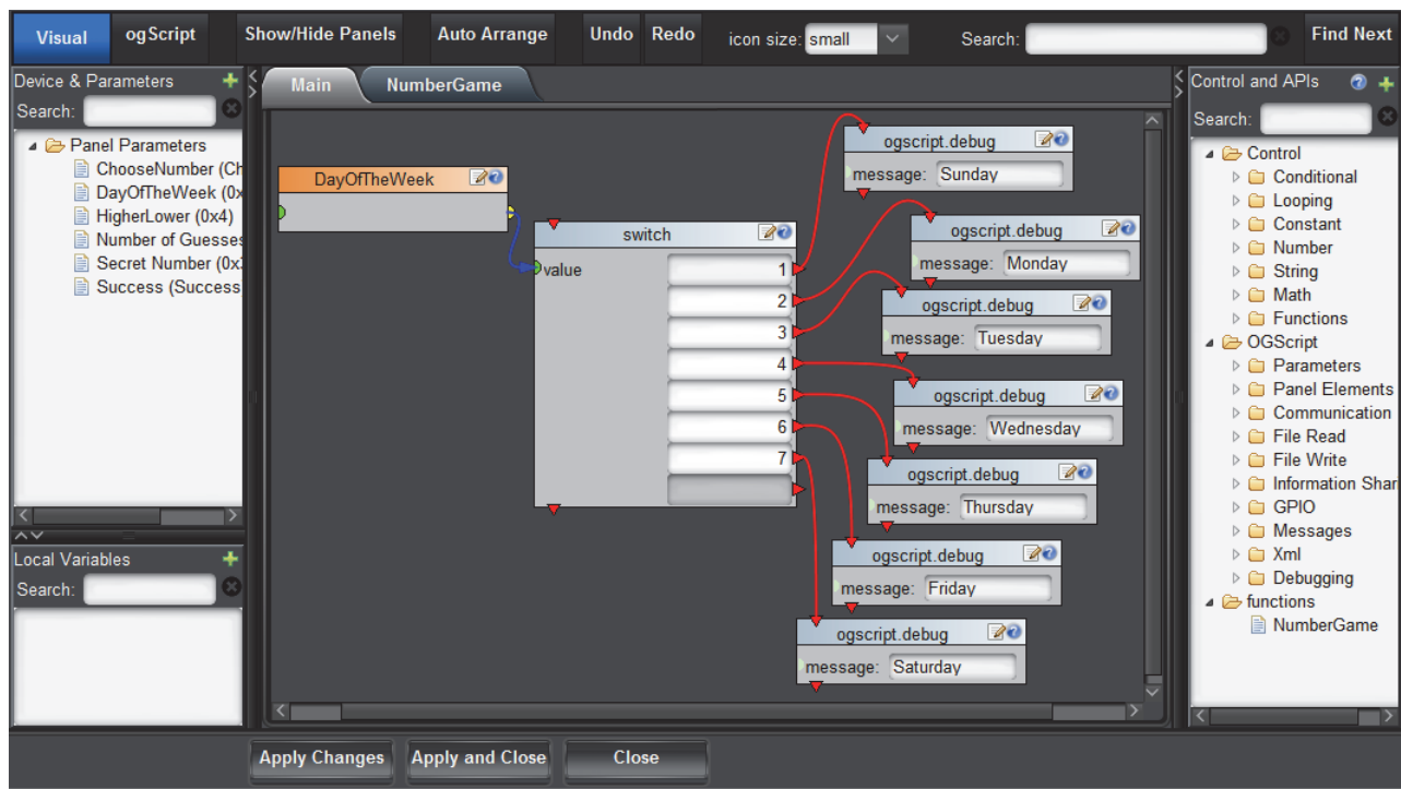
Figure 6.1 - Visual Logic Editor
