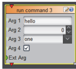
Figure 6.20 - A Block with Each Type of Argument
