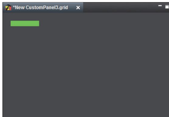
Figure 5.31 - Component anchored to center while panel is expanded
