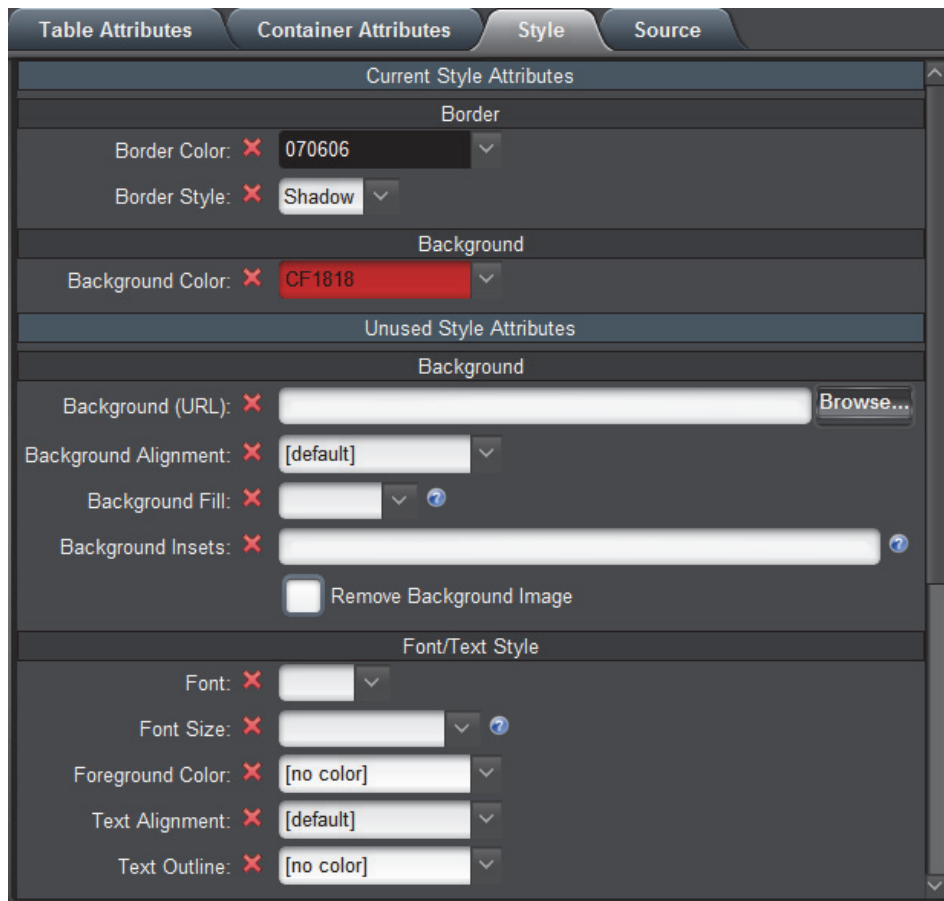
Figure 5.25 - Current and Unused Attributes
