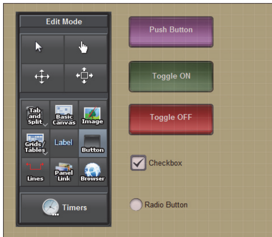
Figure 5.19 - Adding Buttons
