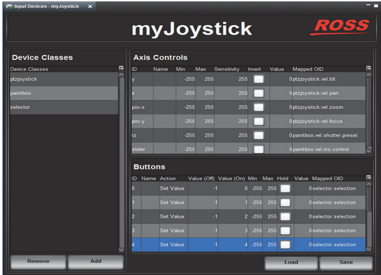
Figure 9.3 - Mapping USB Controller Data to PIVOTCam Control Panel Parameter OIDs
